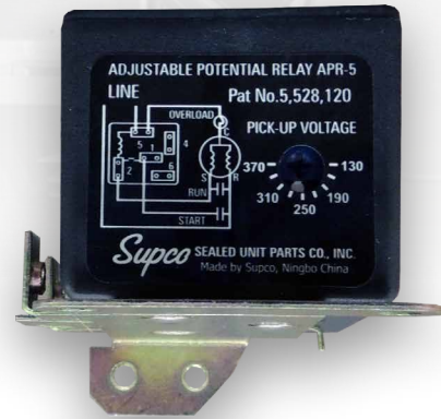
ADJUSTABLE POTENTIAL RELAY APR5
