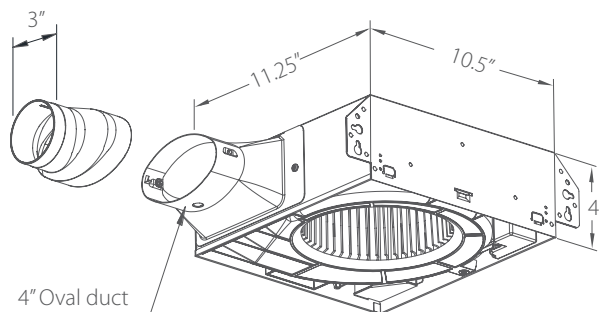
Fan Housing for SLM80 and SLM100
